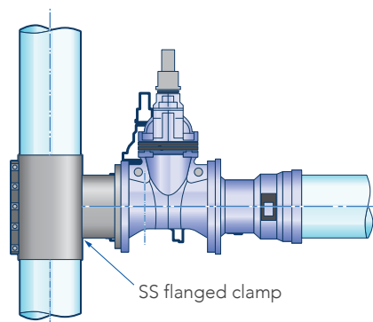
Under pressure cut-in (Utilising stainless steel flanged clamp)
