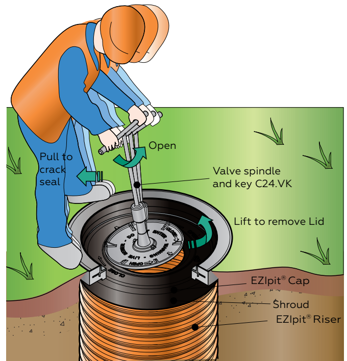
Figure 17: Removing the EziPit Lid from the Cap for Sewer Inspection or Vacuum Testing.
