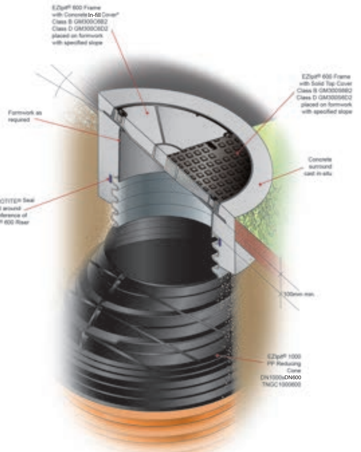
Figure 48: EziPit 1000 MH with GATIC® cover arrangement Class B & D (Sloped Surfaces). Concrete frame cast insitu by others to specified slope.
