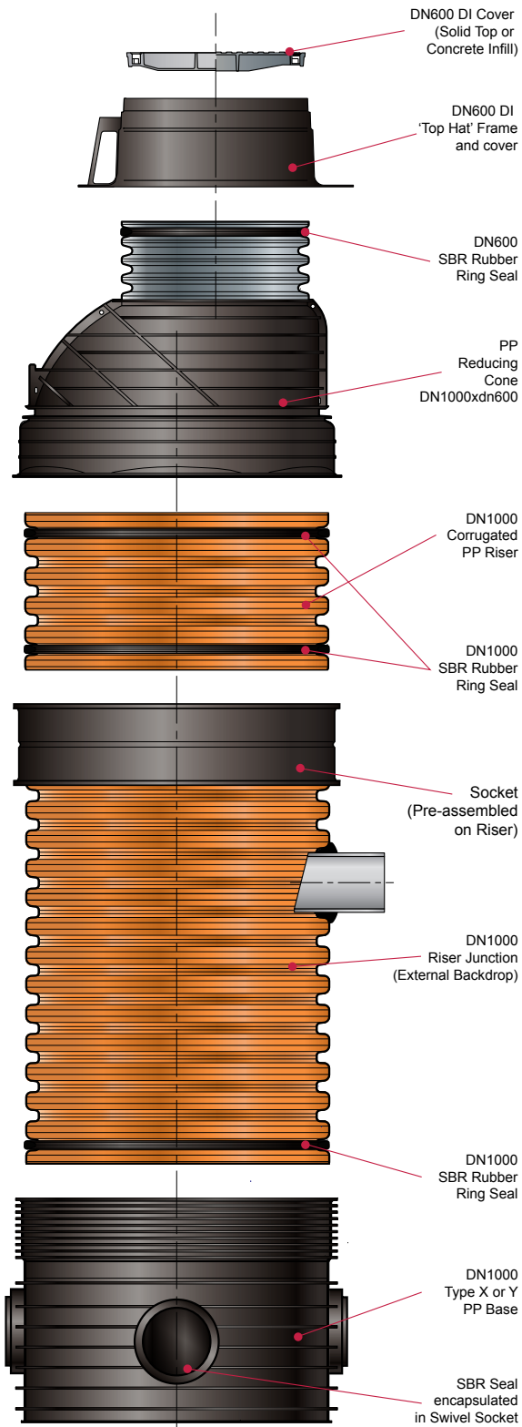
Figure 52: EziPit 1000 Maintenance Hole (MH) assembly with Riser Junction for External Drop
