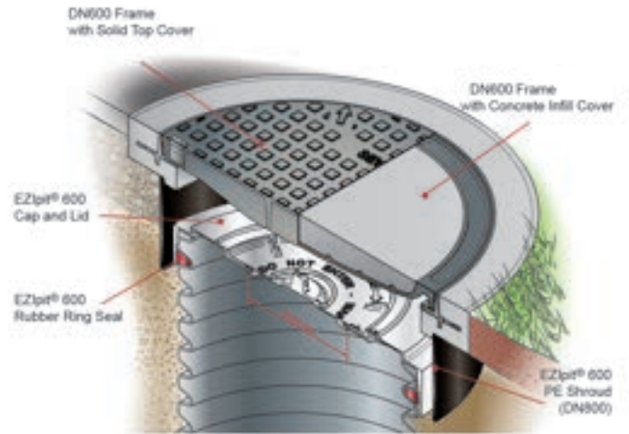
Figure 37: GATIC® EziPit 600 Class B Conventional cover arrangement, assembled with riser.
