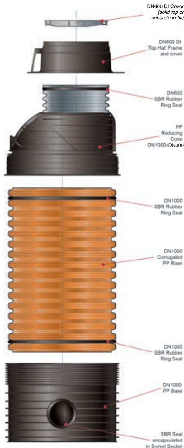
Figure 44: EziPit 1000 Maintenance Hole (MH) assembly
