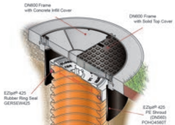
Figure 25: EziPit 425 Cover arrangement (Sloped surfaces).
