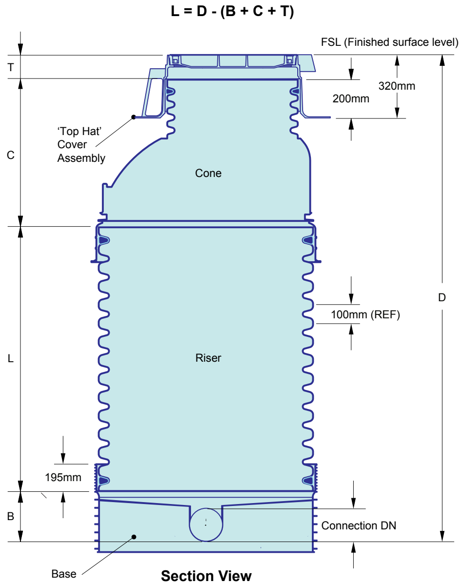
Figure 54: EziPit 1000 MH Assembly
