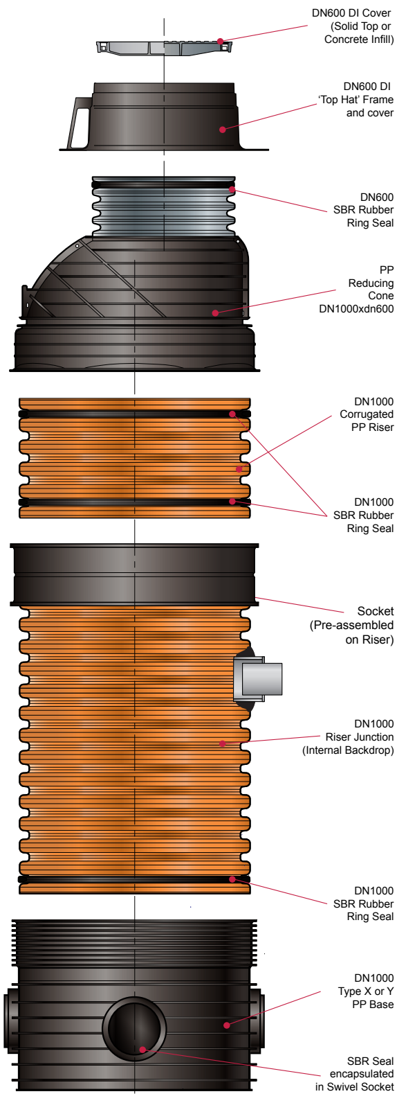
Figure 50: EZiPit 1000 Maintenance Hole (MH) assembly with Riser Junction for Internal Drop
