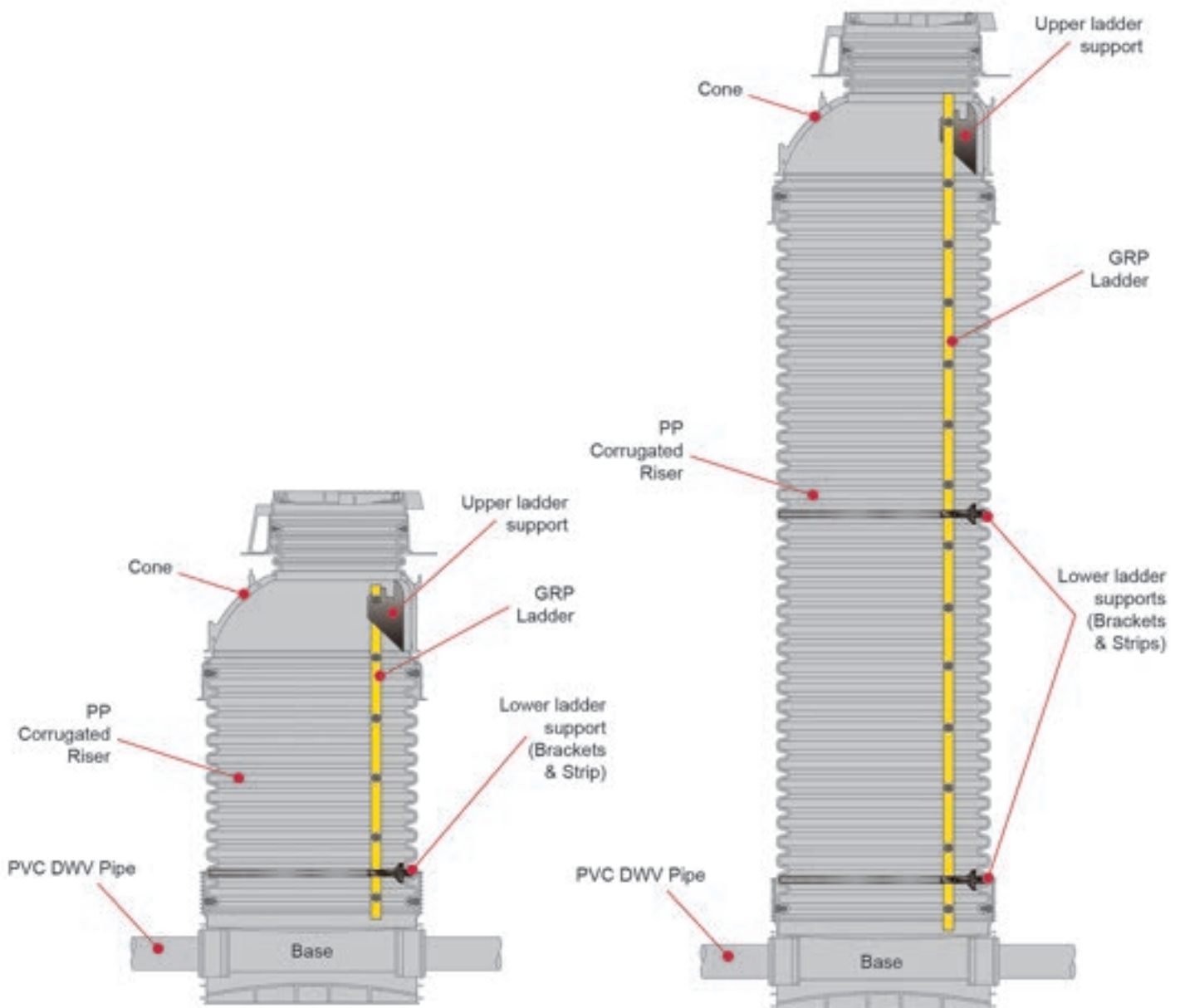
Figure 56: EziPit 1000 MH ladder with one lower ladder support. (Maximum installation depth 3.671m)
