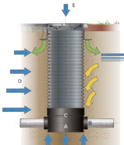
Figure 6: The flexible nature of the EziPit corrugated riser allows a robust structure.
