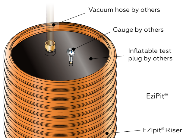
Figure 20: Test plug assembled in EziPit Riser ready for test.
