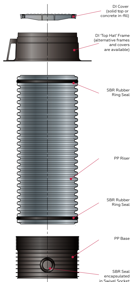
Figure 32: EziPit 600 Maintenance Chamber assembly.
