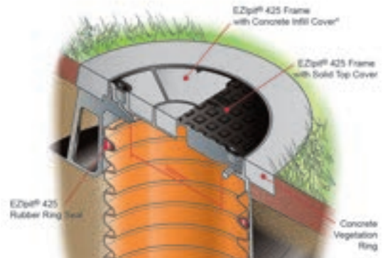
Figure 23: EziPit 425 Class B 'Top Hat' Cover arrangement.
