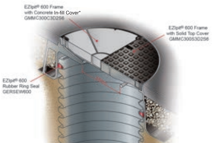
Figure 35: EziPit 600 Class D GATIC® 'Top Hat' cover arrangement, assembled with riser.
