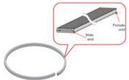
Figure 60: EziPit 1000 Strip
