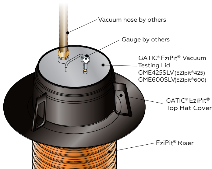
Figure 19: Vacuum Testing using DN425 or 600 GATIC® EziPit Lid with 'Top Hat' Frame.
