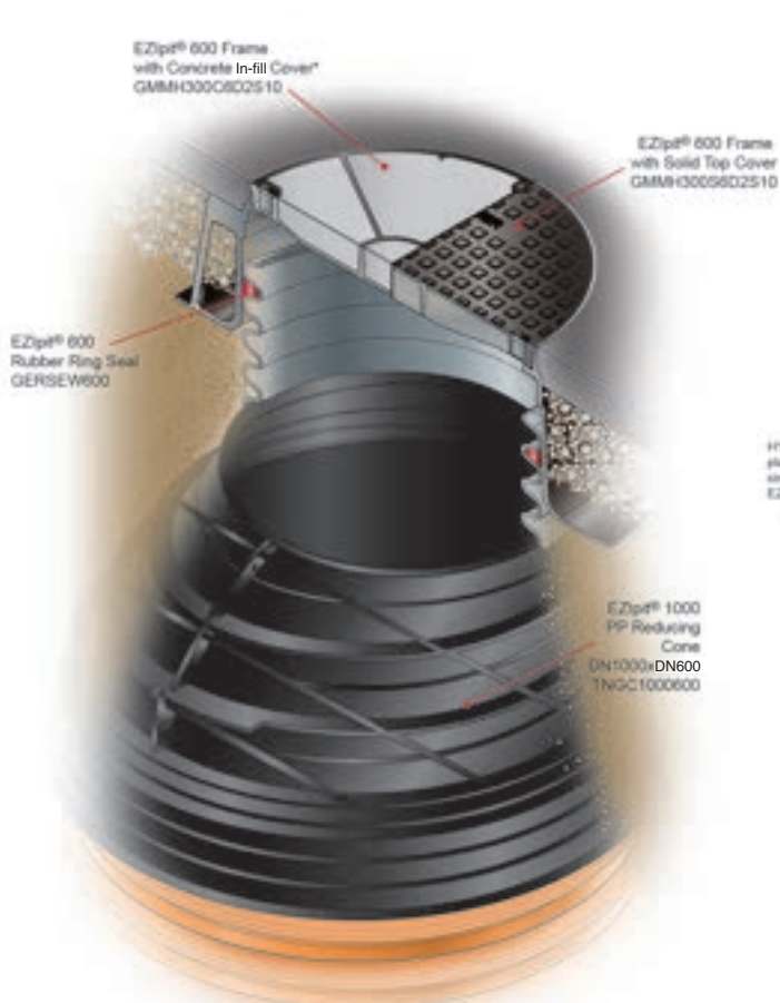
Figure 47: EziPit 1000 MH with GATIC® 'Top Hat' cover arrangement Class D, assembled with riser
