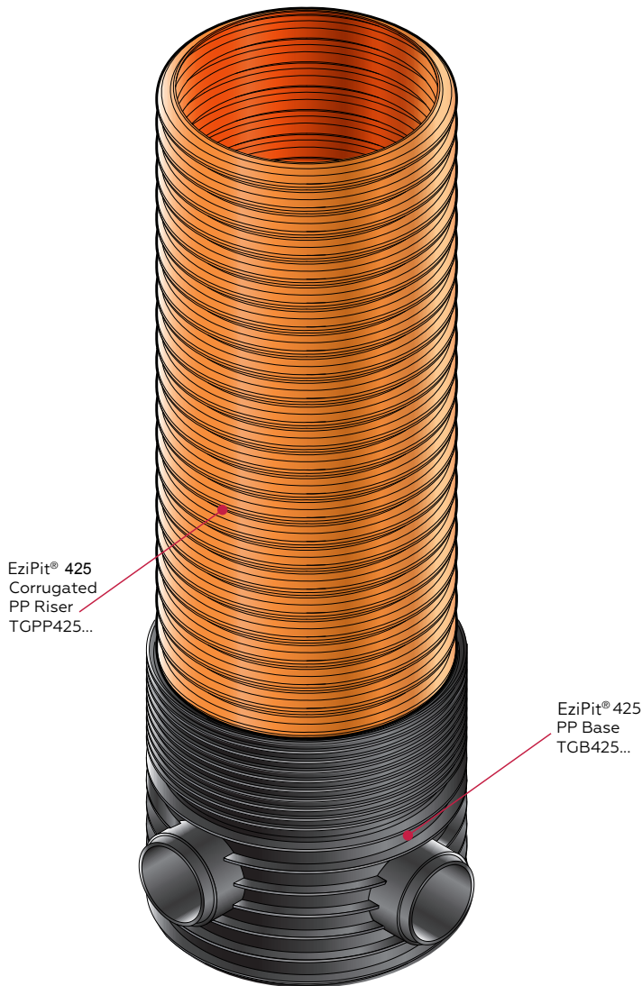
Figure 22: EziPit 425 Base & Riser assembly.
