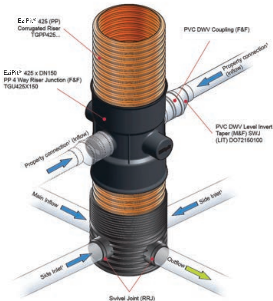
Figure 26: EziPit 425 Maintenance Shaft with lateral sewer connections via the base and the riser.
