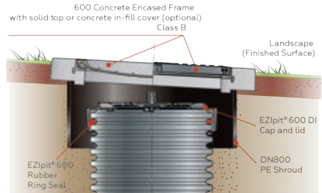
Figure 40: EziPit 600 Cover arrangement (sloped surfaces).
