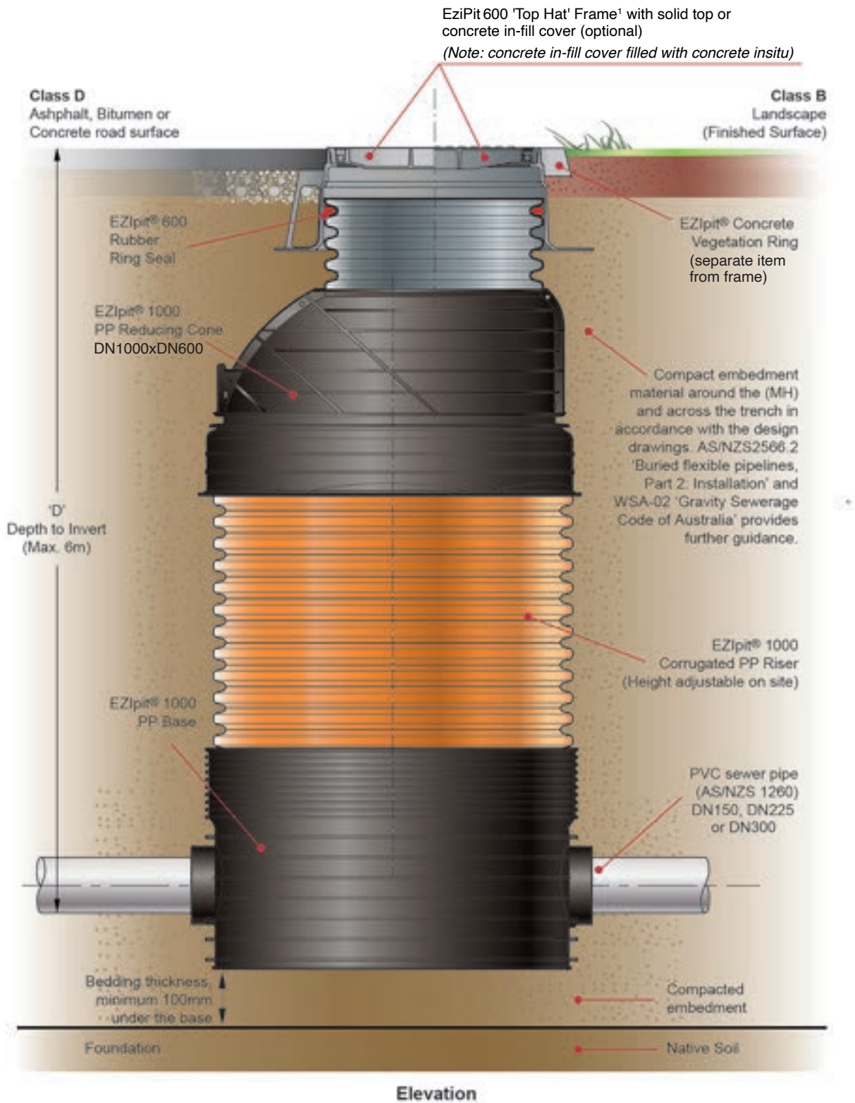
Figure 53: Typical Installation - EziPit 1000 MH with 'Top Hat' Cover Arrangement Class B or D
