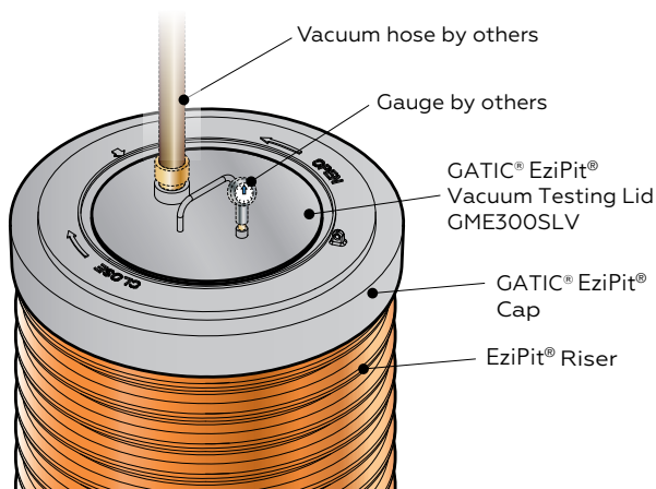
Figure 18: Vacuum testing using DN300 GATIC® EziPit lid with 'cap'.
