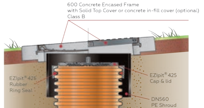
Figure 28: EziPit 425 Cover arrangement (sloped surfaces).
