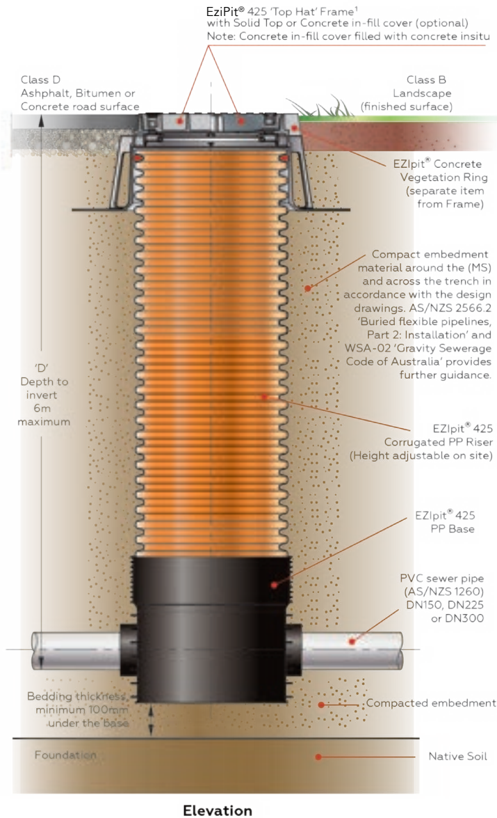
Figure 27: Typical Installation EziPit 425 Maintenance Shaft (MS).
