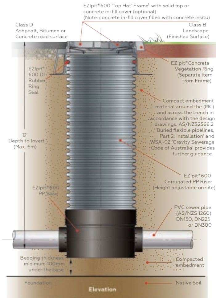
Figure 39: Typical Installation EziPit 600 Maintenance Chamber (MC).
