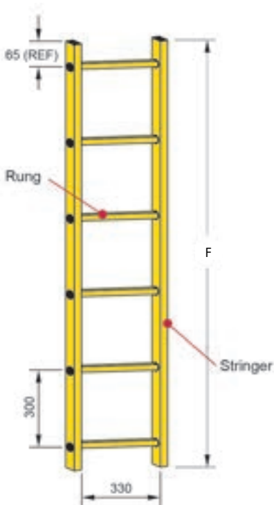
Figure 58 : EziPit 1000 GRP Ladder
