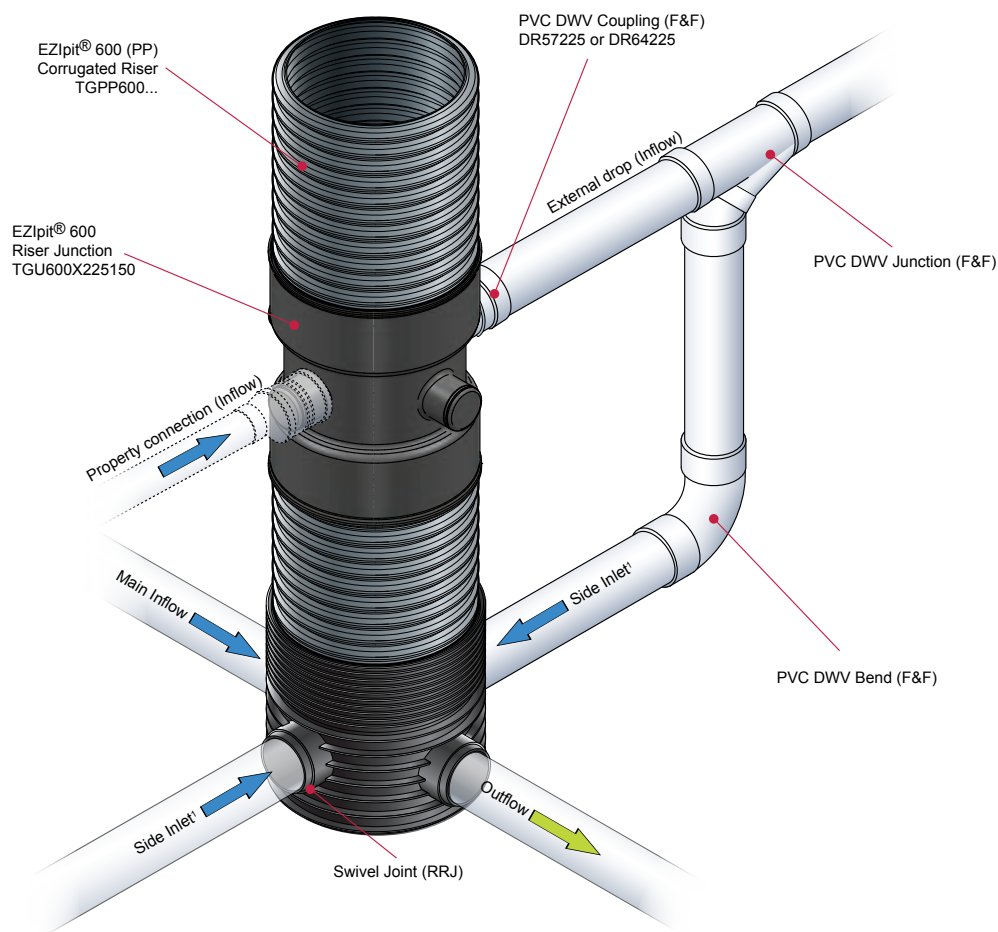
Figure 38: EziPit 600 Maintenance Chamber with Inflow assemblies via the base and the riser. (External Drop) and property connections
