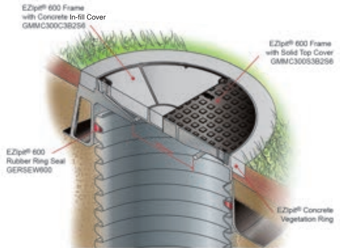
Figure 34: EziPit 600 Class B GATIC® 'Top Hat' cover arrangement, assembled with riser.
