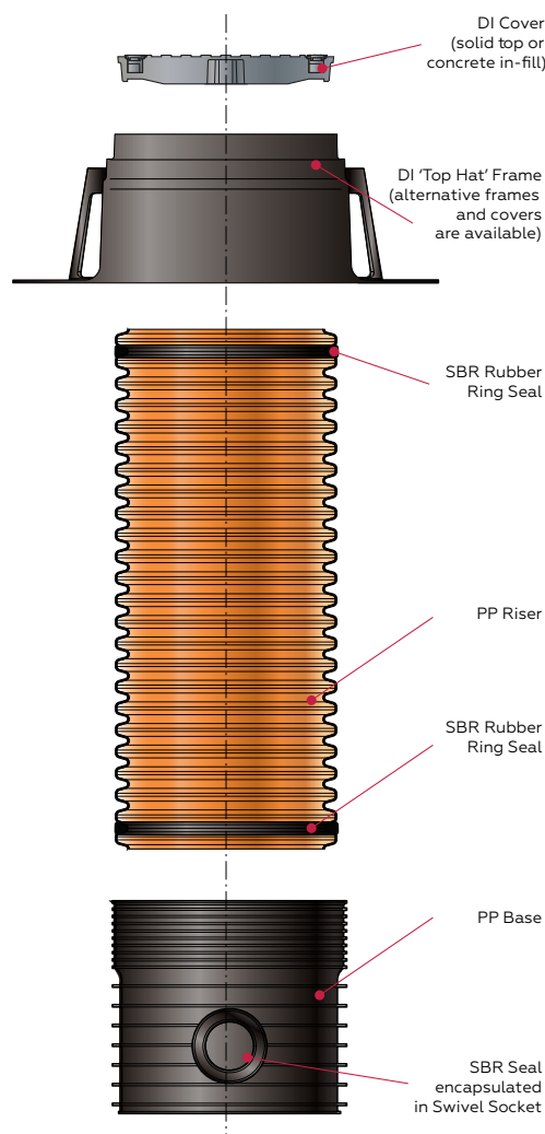
Figure 21: EziPit 425 Maintenance Shaft assembly.
