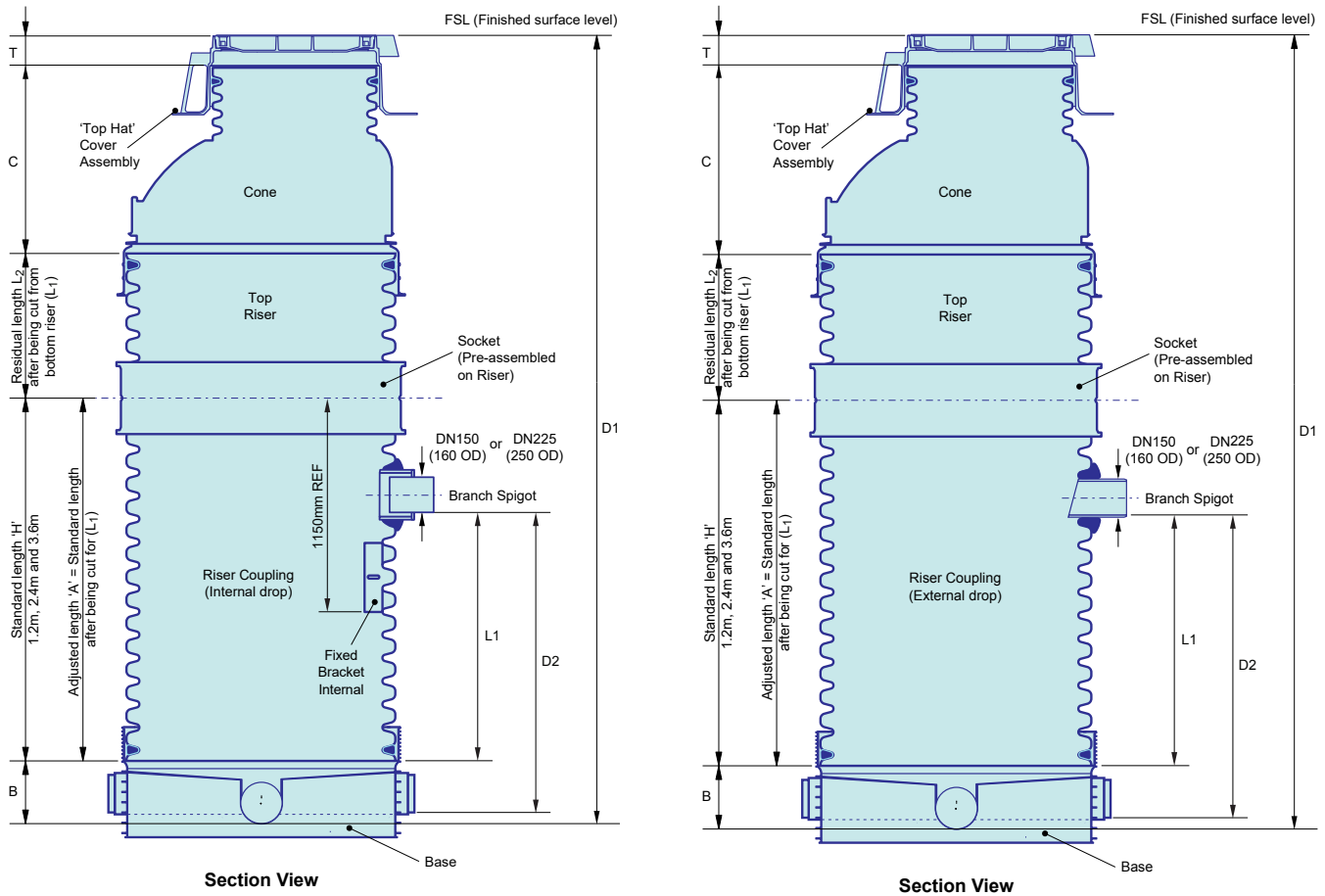
Figure 55: EziPit 1000 MH Assembly with Riser Junction (Branch Connection)
