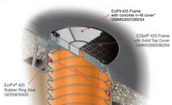
Figure 24: EziPit 425 Class D GATIC® 'Top Hat' Cover arrangement.
