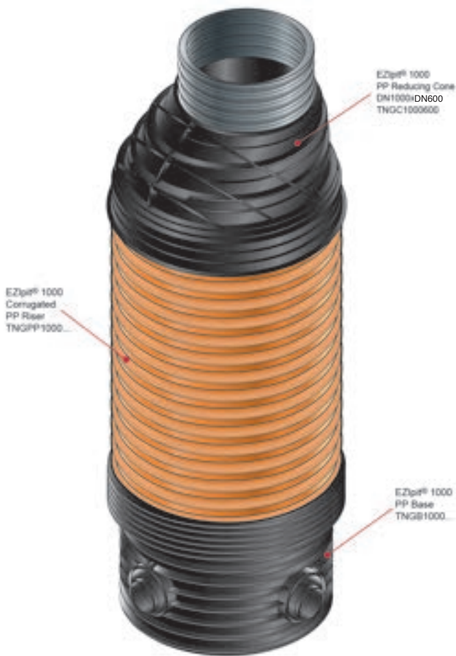
Figure 45: EziPit 1000 Base , Riser and Cone Assembly
