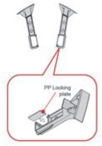
Figure 59: EziPit 1000 GRP Brackets
